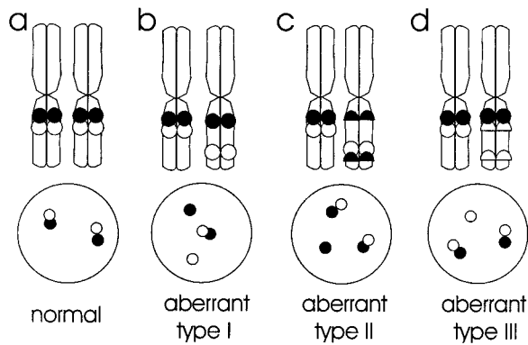
Figure 1. Principle of the interphase FISH assay. PACs centromeric of the 3q21 breakpoint region (closed symbols) were labeled with a red and PACs telomeric of the breakpoint region (open symbols) with a green fluorescent dye. a: Expected hybridization pattern on normal chromosomes 3 and corresponding interphase nuclei. b: Expected hybridization pattern on chromosomes and in interphases with a 3q21 rearrangement whose breakpoint is located at or near a small region of overlap between the red and green labeled PACs (aberrant pattern type I). An inv(3)(q21q26) is depicted in the scheme, but the same interphase patterns would be expected for other 3q21 rearrangements. c,d: Expected hybridization patterns in cells with a more centromeric ( c ) or a more telomeric ( d ) 3q21 breakpoint, which result in split red or green signals, yielding aberrant patterns type II and III, respectively.
